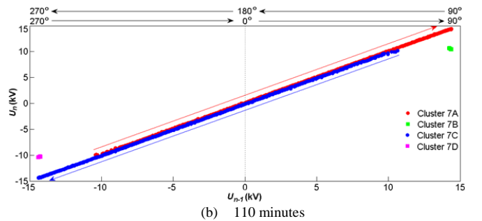
Fig. 3. The consecutive voltage plot, u_n vs u_{n-1} , of PD from a sample tested
