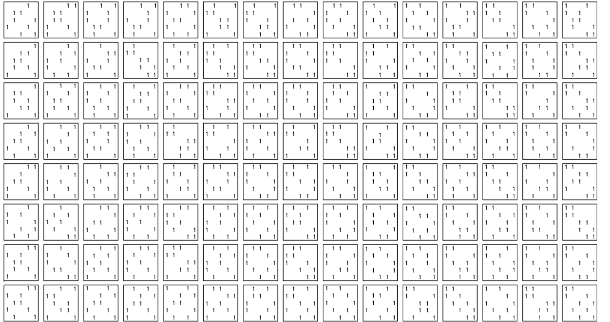
Fig. 3.2. All 5 \times 5 intersection matrices of length 28
