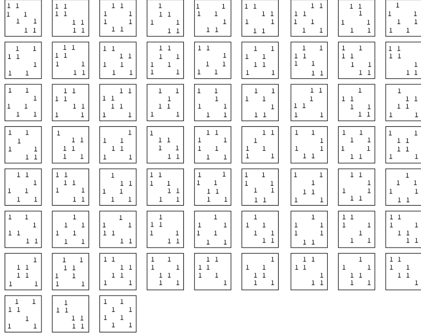
Fig. 3.1. All 4 \times 4 intersection matrices of length 18
